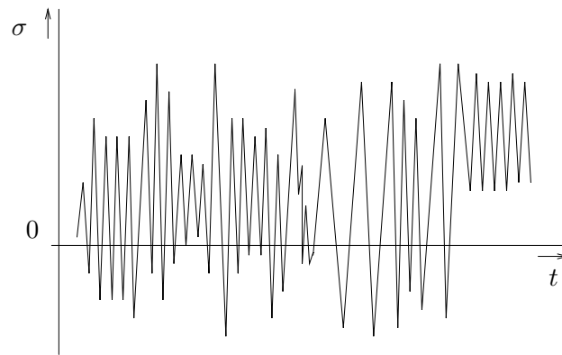
Fig. 12.22 : Random load.
