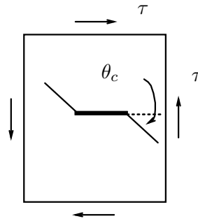
Fig. 7.10 : Crack growth direction for Mode II loading.
