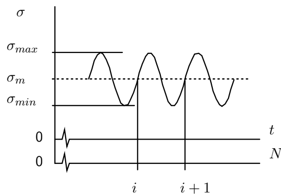
Fig. 12.2 : Harmonic stress.
