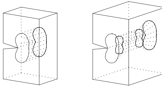
Fig. 9.4 : Plastic crack tip zone for a thin and a thick plate.
