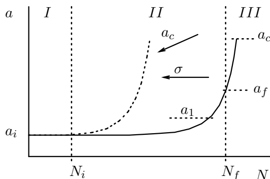
Fig. 12.15 : Crack length increase with number of cycles.
