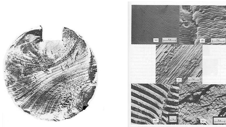
Fig. 12.1 : Clam shell fatigue crack surface and striations [29].
