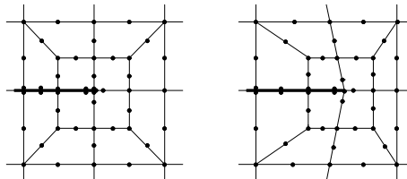
Fig. 11.9 : VCEM in crack tip mesh.
