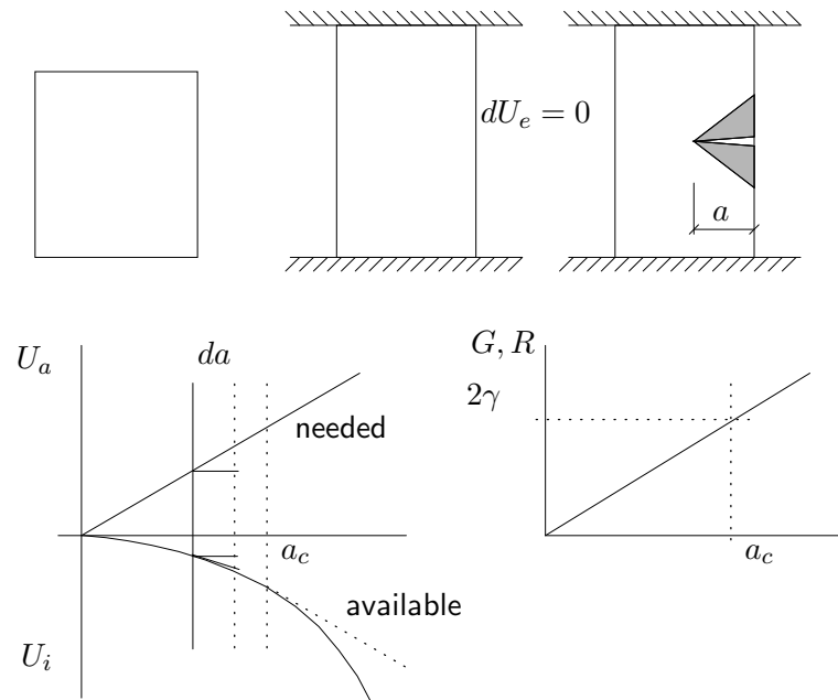
Fig. 4.2 : Illustration of Griffith's energy balance criterion.
