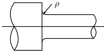
Fig. 12.12 : Stress concentration at axis diameter reduction.
