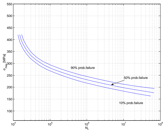
Fig. 12.7 : P-S-N-curves.
