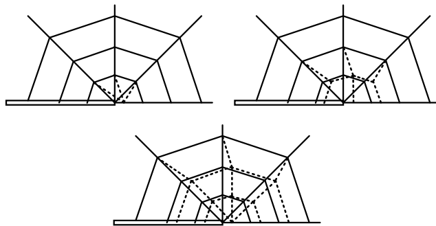
Fig. 11.14 : J-integral domain with various element rings.
