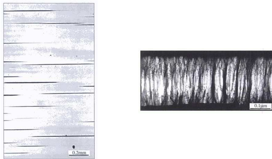
Fig. 2.4 : Crazes in polystyrene on a macroscopic and microscopic scale. (Source: Internet)
