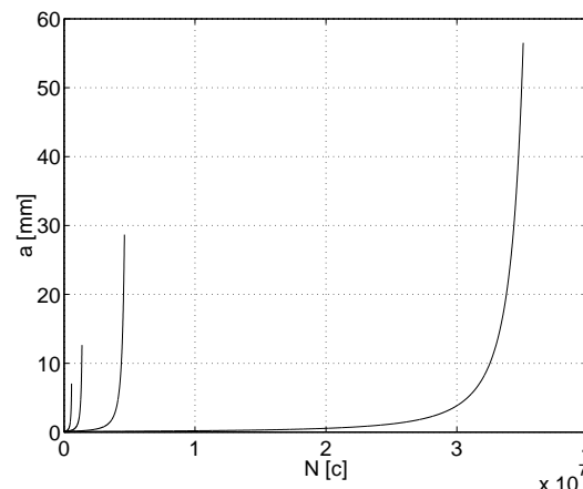
Fig. 12.19 : Fatigue crack length in aluminum for various load amplitudes.
